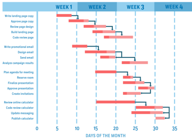
Figure 1: Gantt chart
