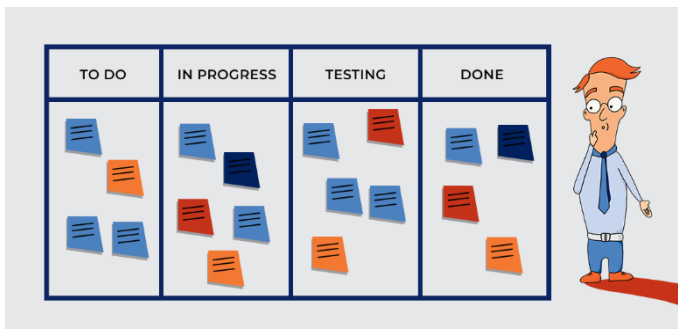
Figure 3: Kanban
